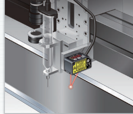
Controlling the dispenser head height
