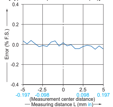
■ Linearity characteristics [Typical example: HG-C1030(-P)]
