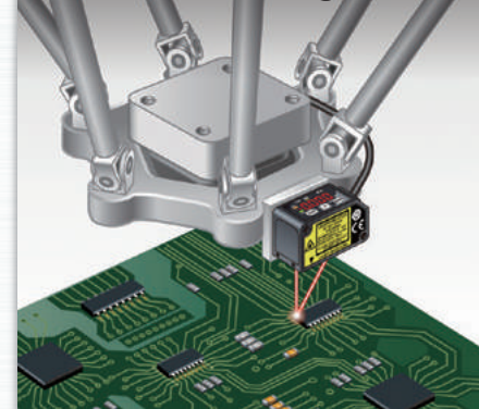
Controlling the parallel link robot height
